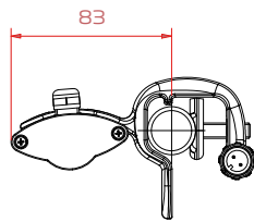
Clamp flipped for circular section
